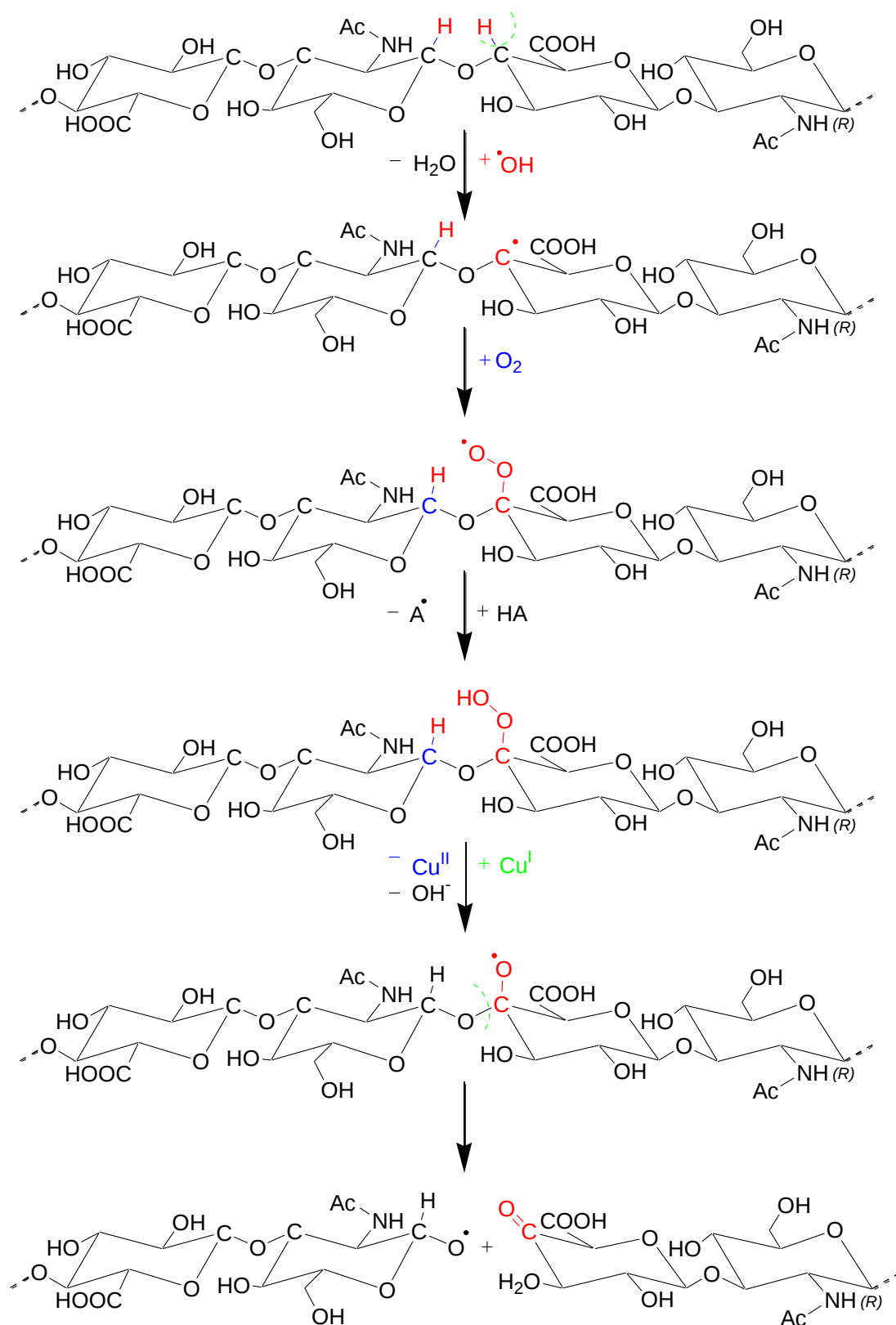
Fig. 4: Schematic degradation of HA under free radical stress (Hrabarova et al. , 2012).
