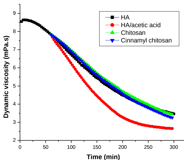
Fig. 6: Effect of chitosan and Cinnamyl chitosan dissolved in acetic acid (0.5%) on the hyaluronan degradation induced by WBOS (black) when added to the reaction system after 1 hour of initiating the degradation of HA
