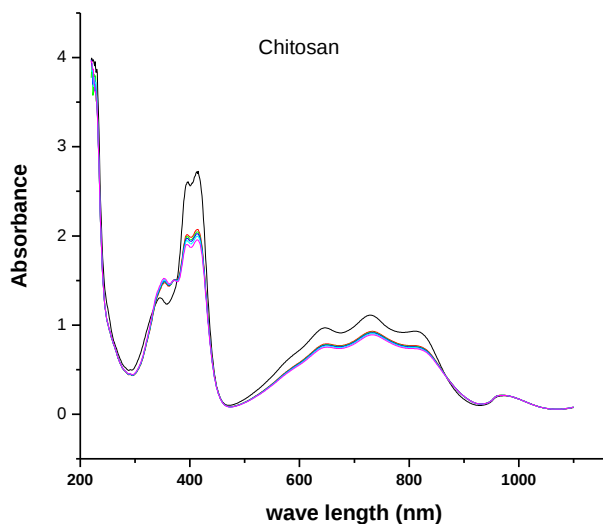
Fig. 7: Effect of Chitosan and cinnamyl chitosan (conc. 0.125 mg/ml) on reducing ABTS + cation radical.
