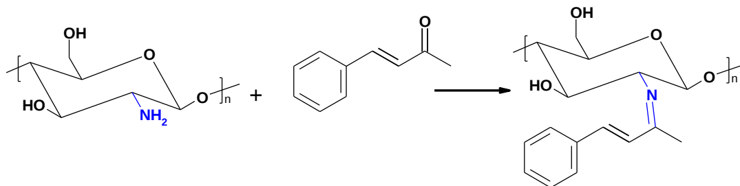
Fig. 2: Schematic preparation of Cinnamyl chitosan from chitosan.
