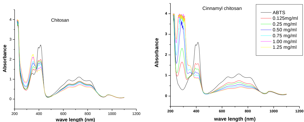
Fig. 9: Effect of Chitosan and cinnamyl chitosan concentration on reducing ABTS^{++} cation radical measured 10 min after the reaction onset.
