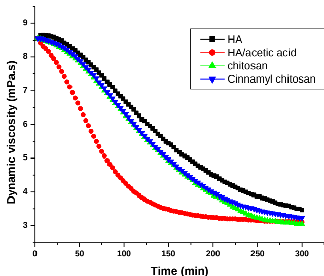
Fig. 5: Effect of chitosan and Cinnamyl chitosan dissolved in acetic acid (0.5%) on the hyaluronan degradation induced by WBOS (black) when added to the reaction system before initiating the degradation of HA
