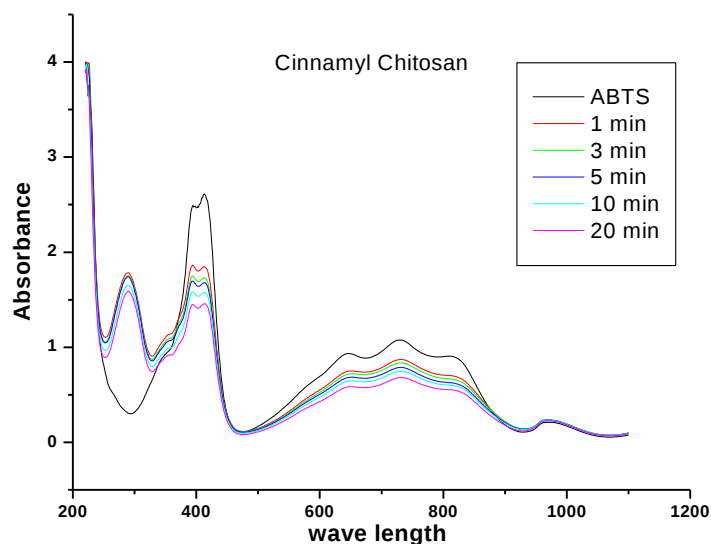
Fig. 7: Effect of Chitosan and cinnamyl chitosan (conc. 0.125 mg/ml) on reducing ABTS + cation radical.
