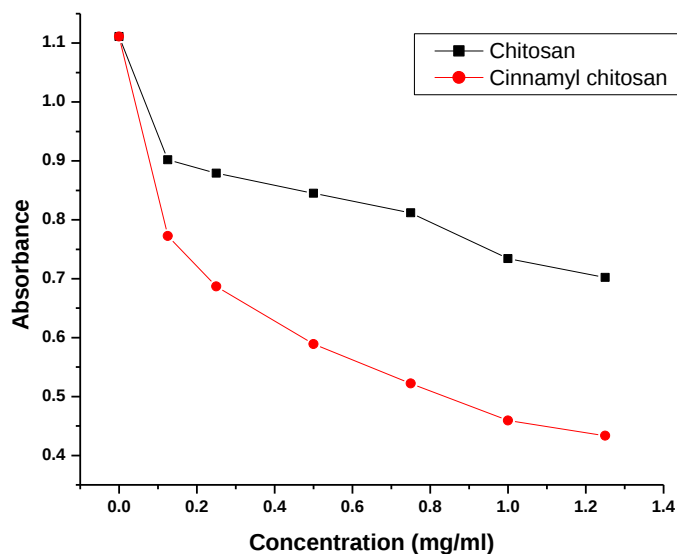
Fig. 10: dose dependency of ABTS^{++} cation scavenging activity of Chitosan and cinnamyl chitosan measured 10 min after the reaction onset.
