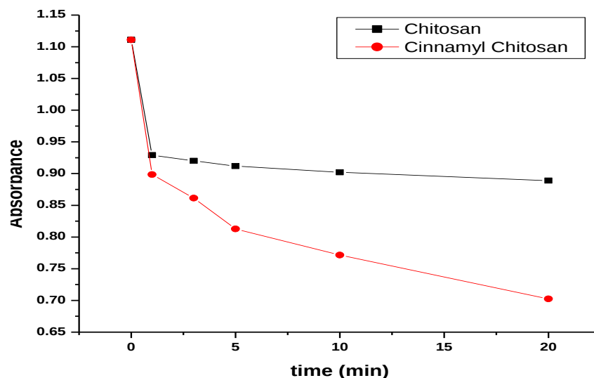
Fig. 8: Time dependence of absorbance at 730 nm measured after addition of polymer solution into the ABTS^{++}
