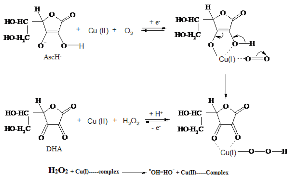
Fig. 3: Weissberger's biogenic oxidation system (WBOS) (Fisher and Naughton., 2005).
